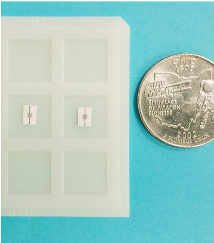
Glenn's microsensor is small and easy to fabricate
